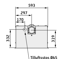
Dimensions from above
