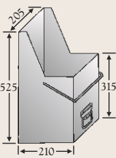
Air vent Part No. 02118
